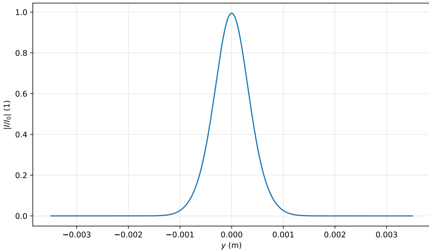
Intensity profile I(x=0, y, z=0.955)/I_0 , P_{in}=0.4P_{cr} , artificial time
